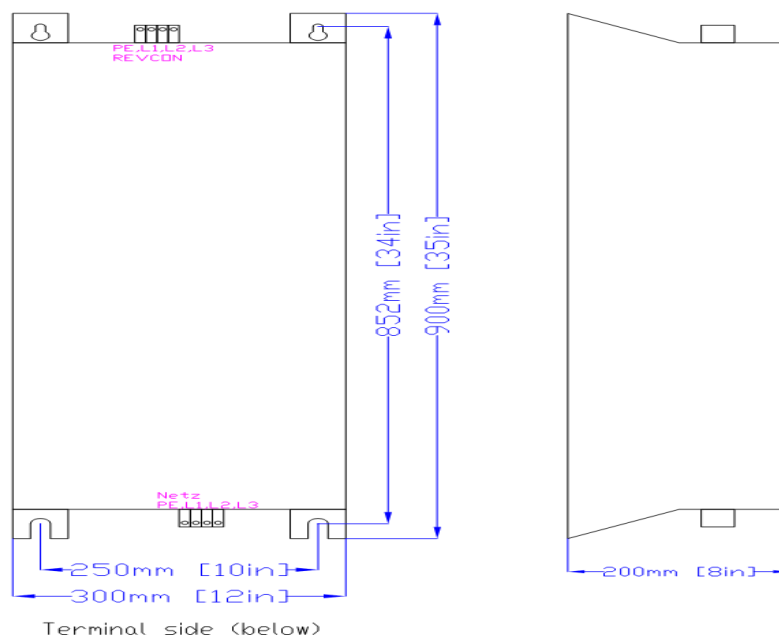
Interference filter construction 3
