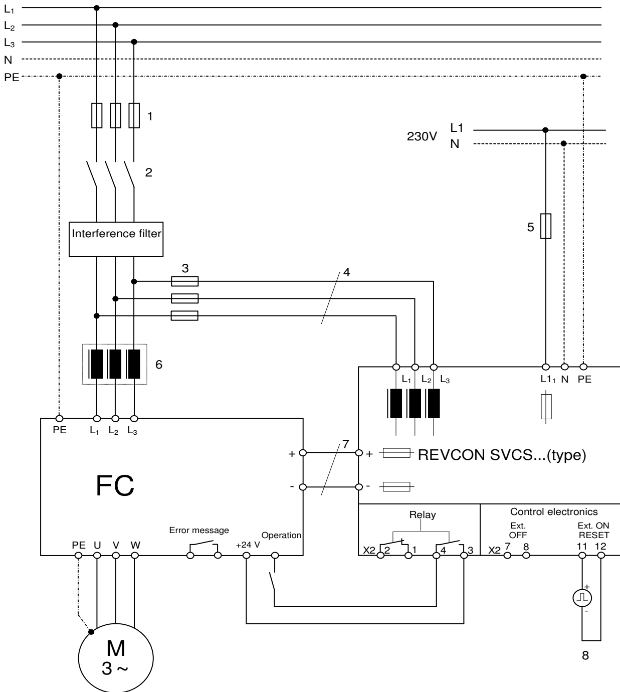
Figure 4.4.1.1.1 Wiring schematic of the power feedback unit REVCON® SVC(S) and one or more controllers
